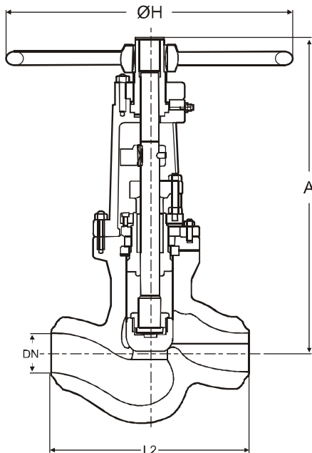
Pressure Seal Globe Valve Class 900/ 1500/ 2500
