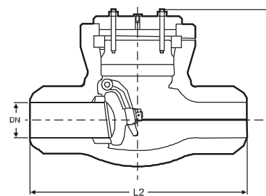
Pressure Seal Swing Check Valve Class 900/ 1500/ 2500
