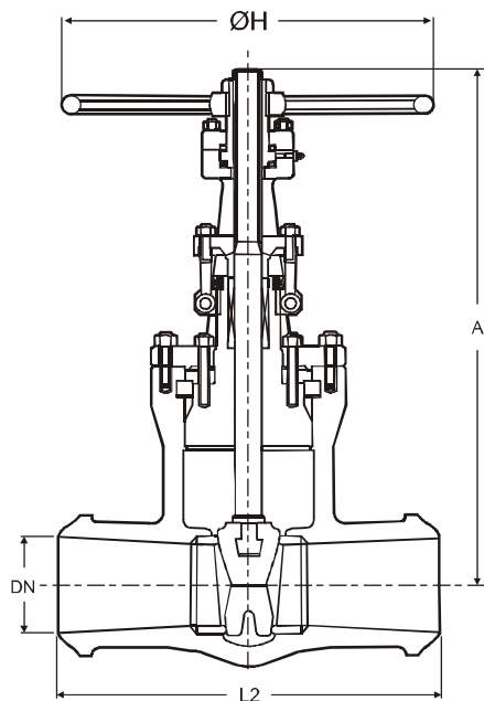
Pressure Seal Gate Valve Class 900/ 1500/ 2500
