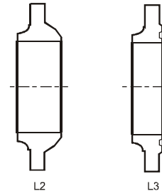
Butt-Weld End
